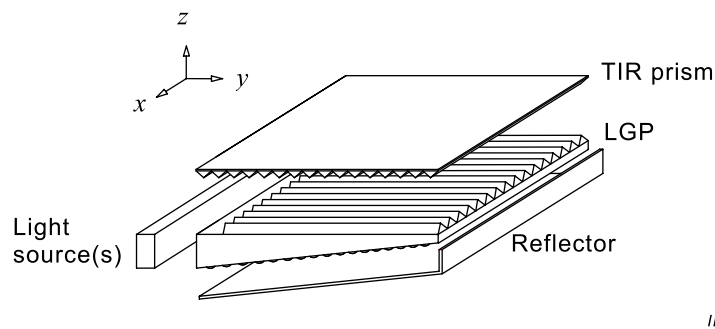
b) Edge-lit backlight unit with TIR prism (an inverted prism with TIR characteristics) and a functional light guide plate
